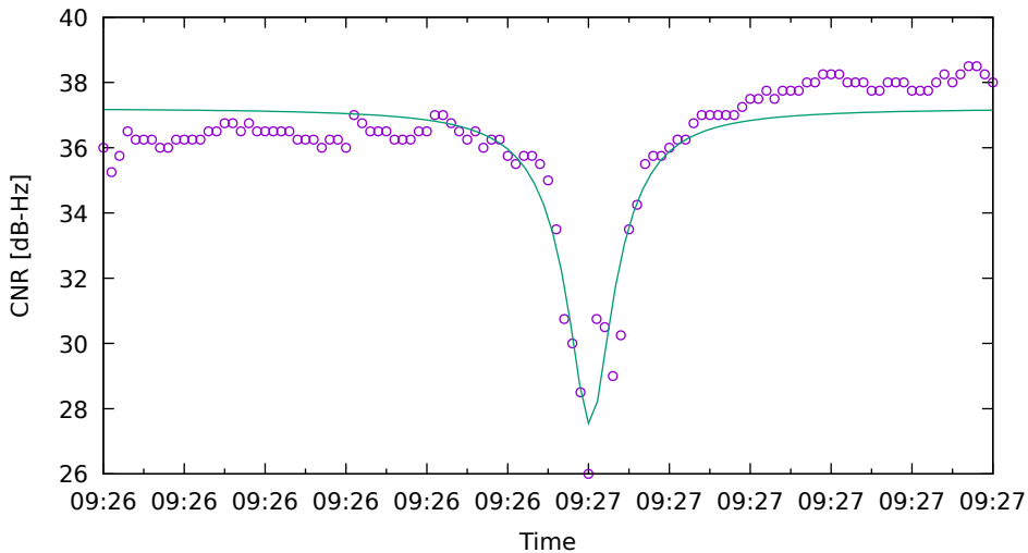
CNR fit for C11 on XiaomiMi8 - drive 6 (DOY262)
