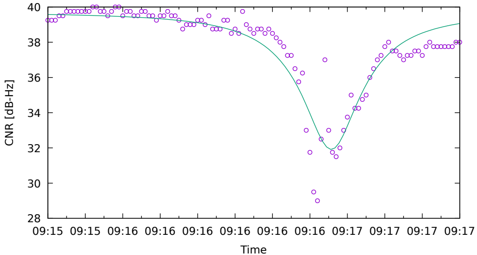
CNR fit for C27 on XiaomiMi8 - drive 1 (DOY262)
