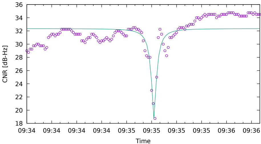
CNR fit for C27 on XiaomiMi8 - drive 10 (DOY262)
