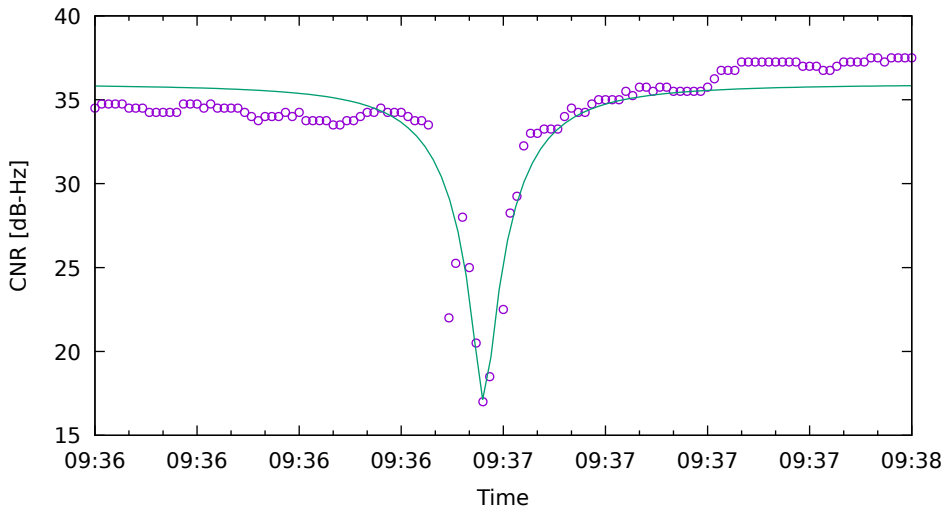
CNR fit for C27 on XiaomiMi8 - drive 11 (DOY262)
