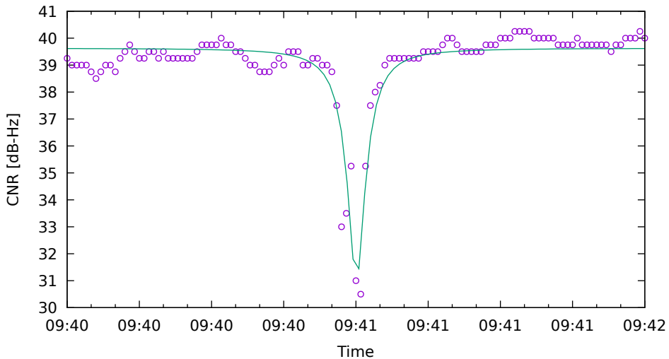
CNR fit for C27 on XiaomiMi8 - drive 13 (DOY262)
