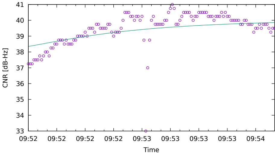
CNR fit for C27 on XiaomiMi8 - drive 19 (DOY262)
