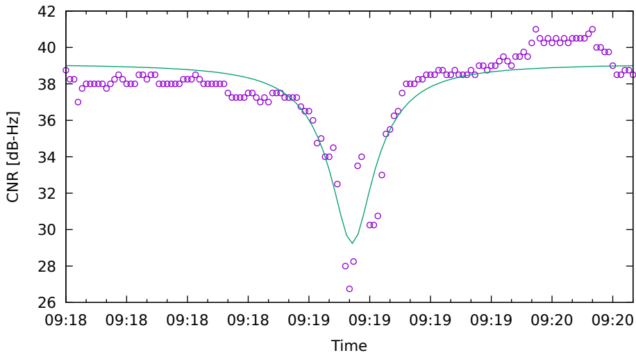
CNR fit for C27 on XiaomiMi8 - drive 2 (DOY262)
