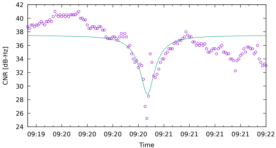
CNR fit for C27 on XiaomiMi8 - drive 3 (DOY262)
