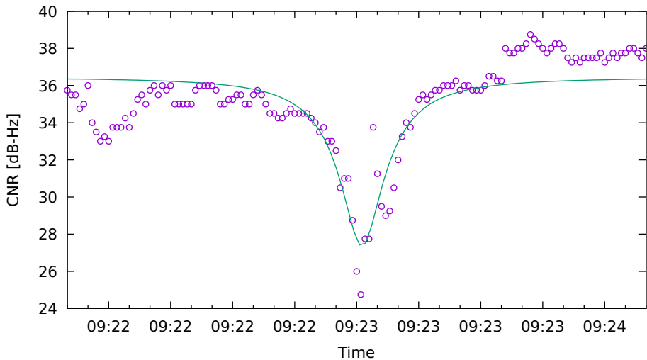
CNR fit for C27 on XiaomiMi8 - drive 4 (DOY262)
