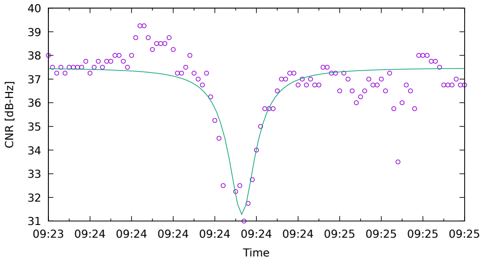
CNR fit for C27 on XiaomiMi8 - drive 5 (DOY262)
