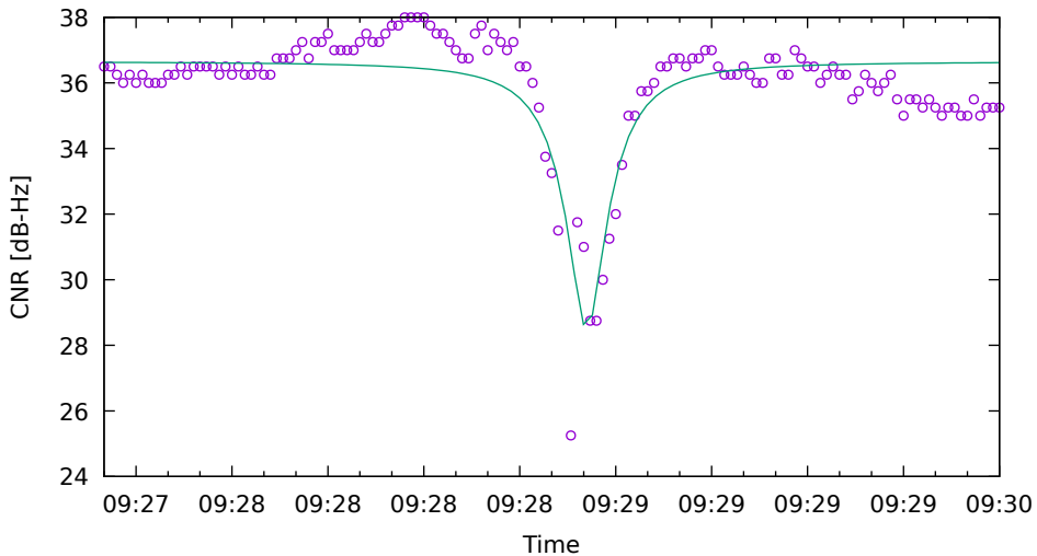
CNR fit for C27 on XiaomiMi8 - drive 7 (DOY262)
