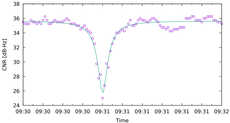
CNR fit for C27 on XiaomiMi8 - drive 8 (DOY262)
