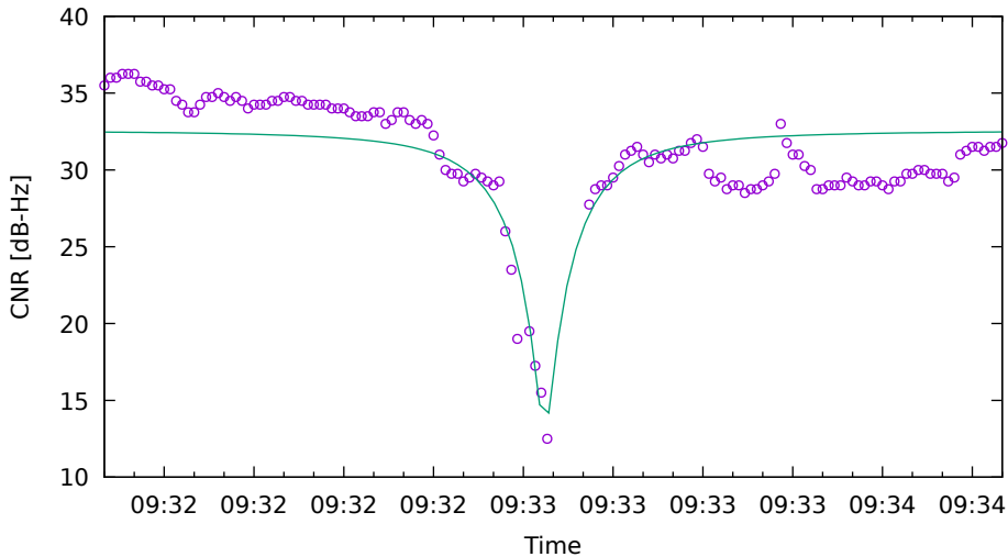
CNR fit for C27 on XiaomiMi8 - drive 9 (DOY262)
