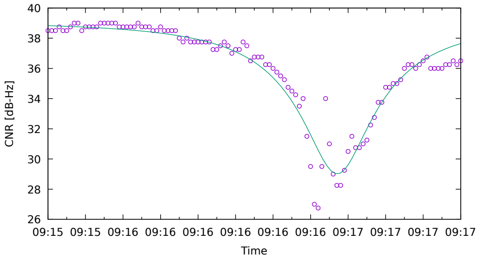
CNR fit for C33 on XiaomiMi8 - drive 1 (DOY262)
