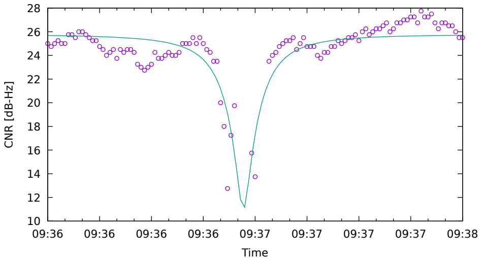
CNR fit for C33 on XiaomiMi8 - drive 11 (DOY262)
