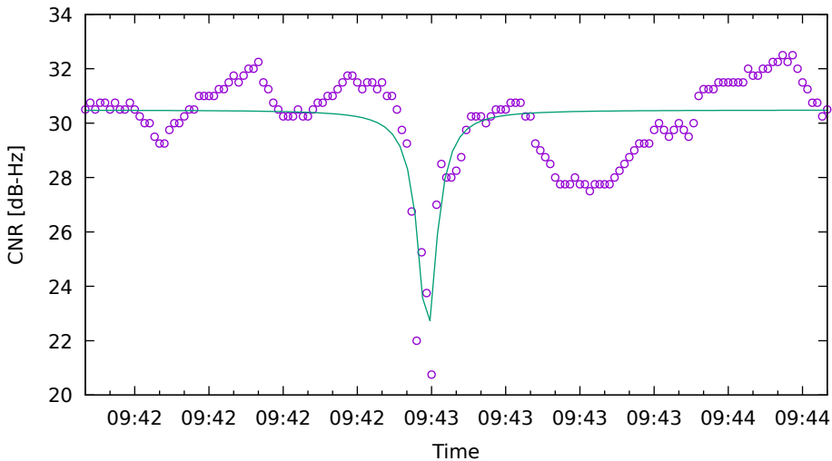
CNR fit for C33 on XiaomiMi8 - drive 14 (DOY262)
