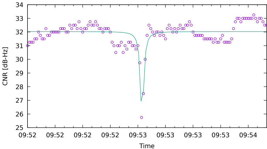
CNR fit for C33 on XiaomiMi8 - drive 19 (DOY262)
