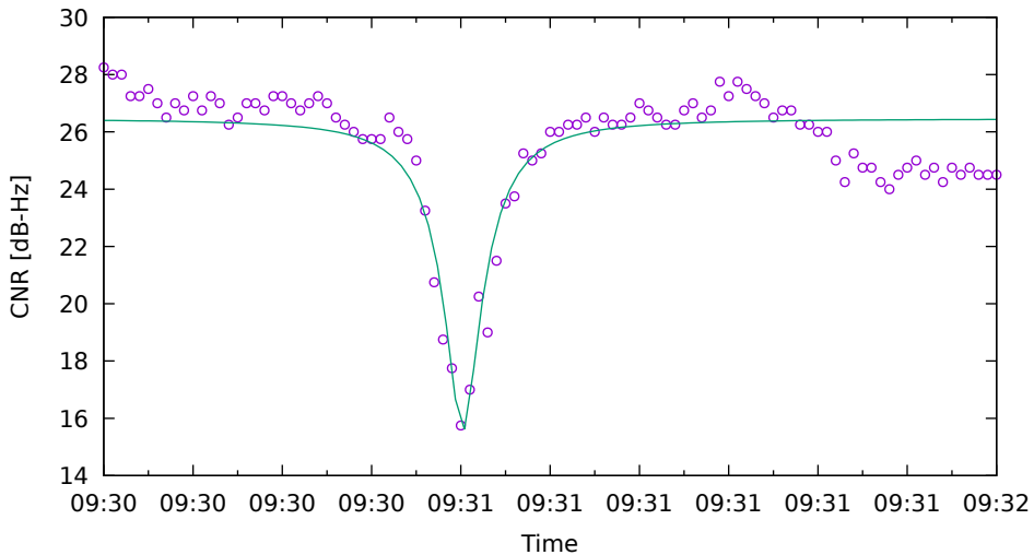
CNR fit for C33 on XiaomiMi8 - drive 8 (DOY262)
