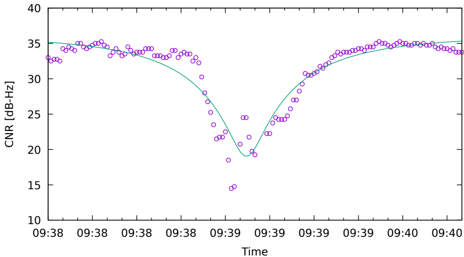
CNR fit for E04 on XiaomiMi8 - drive 12 (DOY262)
