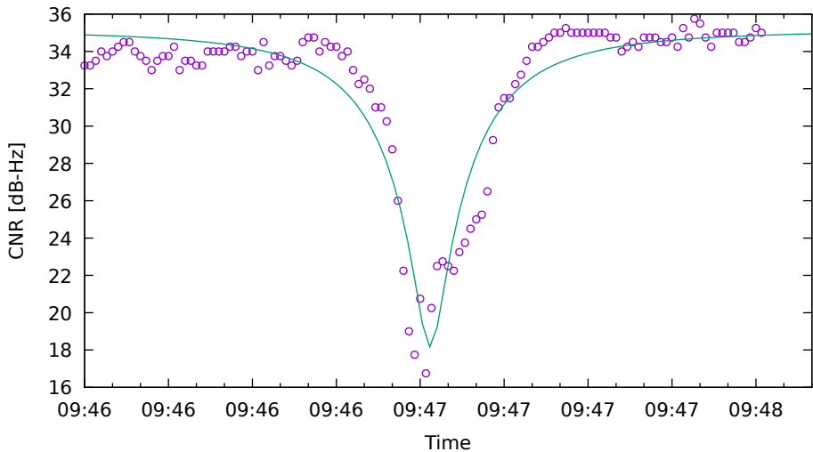
CNR fit for E04 on XiaomiMi8 - drive 16 (DOY262)
