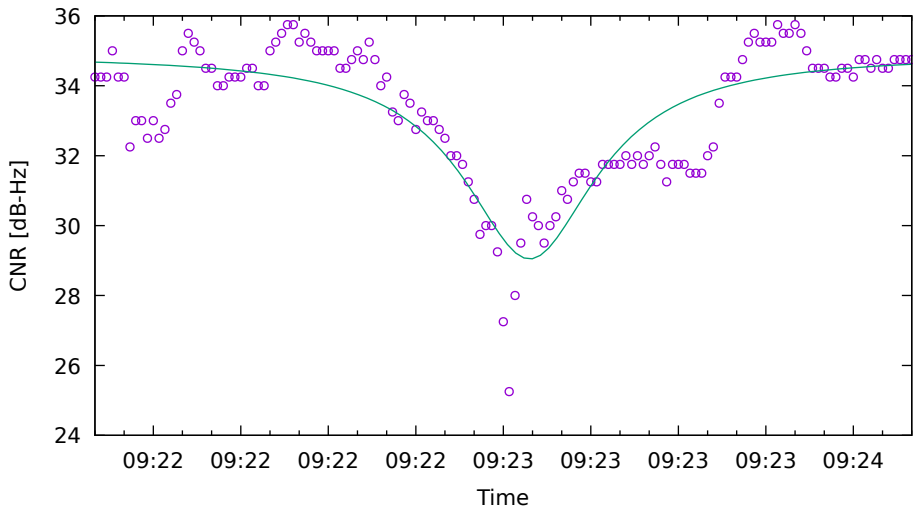
CNR fit for E04 on XiaomiMi8 - drive 4 (DOY262)
