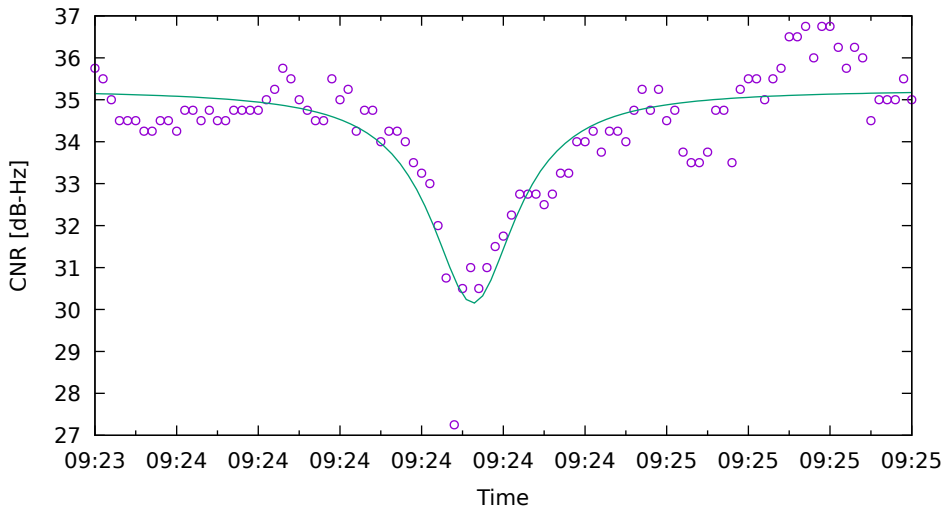
CNR fit for E04 on XiaomiMi8 - drive 5 (DOY262)
