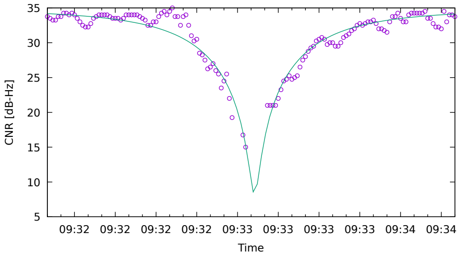
CNR fit for E04 on XiaomiMi8 - drive 9 (DOY262)
