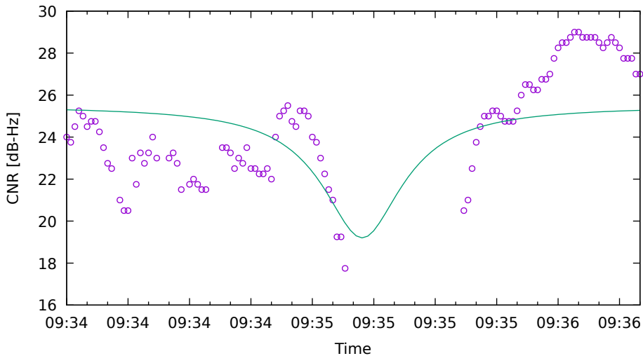
CNR fit for E05 on XiaomiMi8 - drive 10 (DOY262)
