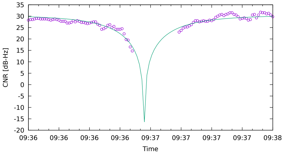
CNR fit for E05 on XiaomiMi8 - drive 11 (DOY262)
