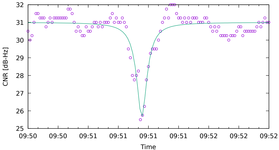
CNR fit for E05 on XiaomiMi8 - drive 18 (DOY262)
