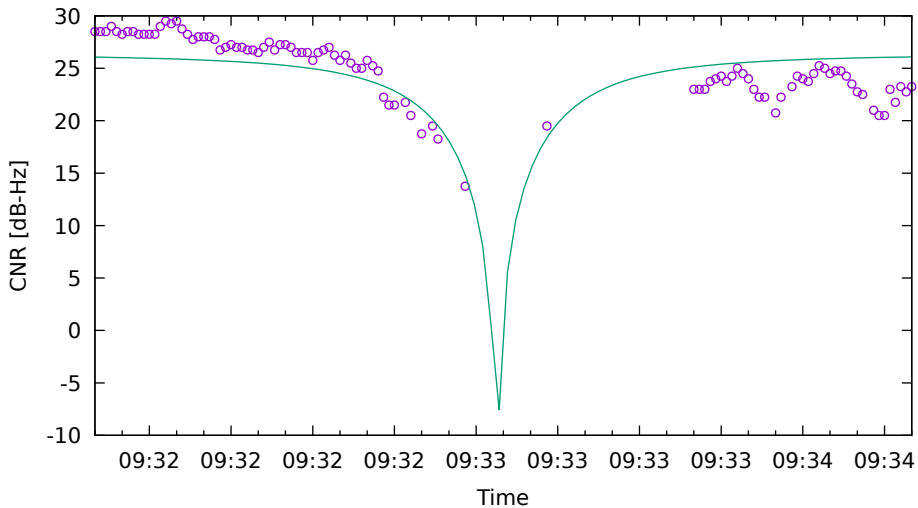
CNR fit for E05 on XiaomiMi8 - drive 9 (DOY262)
