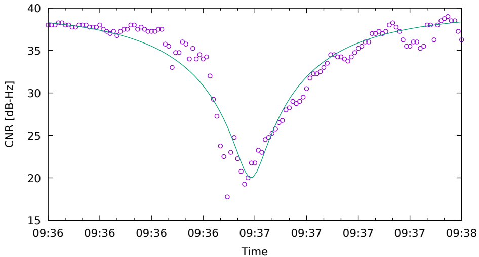
CNR fit for E09 on XiaomiMi8 - drive 11 (DOY262)
