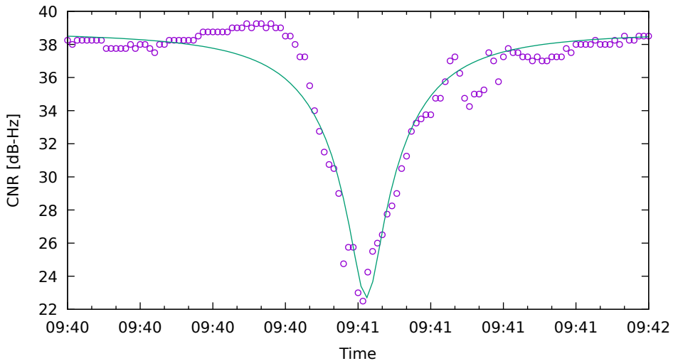
CNR fit for E09 on XiaomiMi8 - drive 13 (DOY262)
