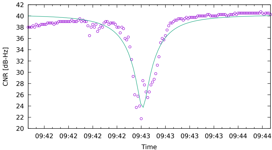
CNR fit for E09 on XiaomiMi8 - drive 14 (DOY262)
