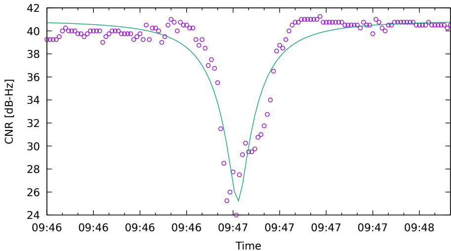
CNR fit for E09 on XiaomiMi8 - drive 16 (DOY262)
