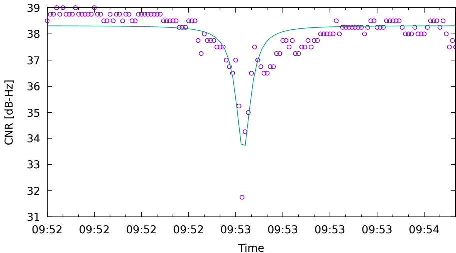
CNR fit for E09 on XiaomiMi8 - drive 19 (DOY262)
