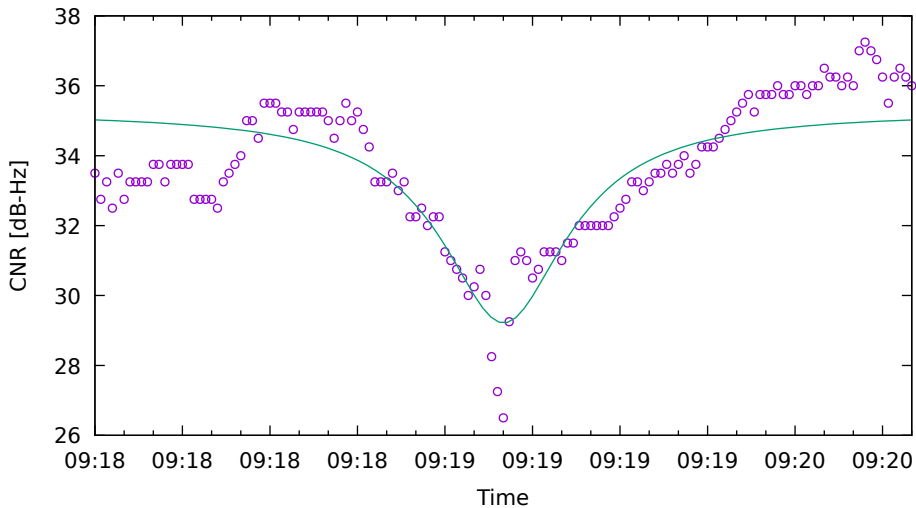
CNR fit for E09 on XiaomiMi8 - drive 2 (DOY262)
