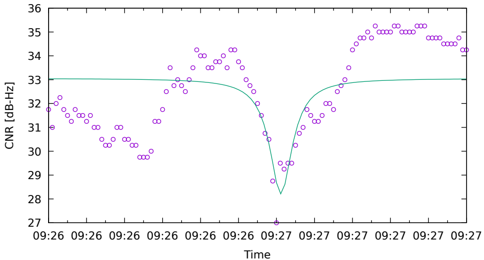
CNR fit for E09 on XiaomiMi8 - drive 6 (DOY262)
