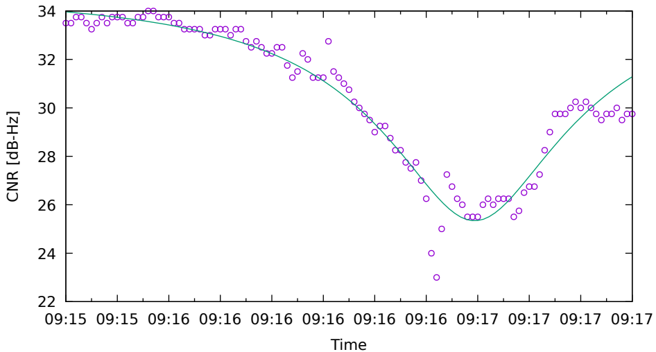
CNR fit for E34 on XiaomiMi8 - drive 1 (DOY262)
