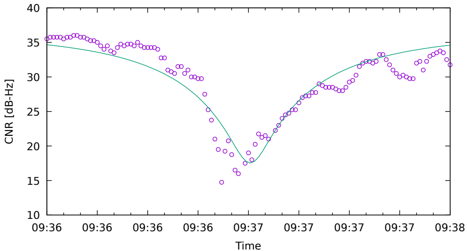
CNR fit for E34 on XiaomiMi8 - drive 11 (DOY262)
