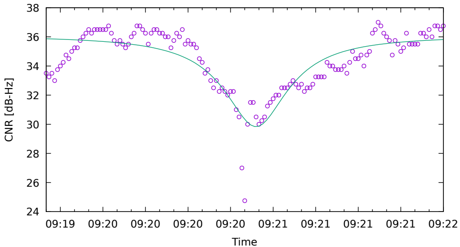
CNR fit for E34 on XiaomiMi8 - drive 3 (DOY262)
