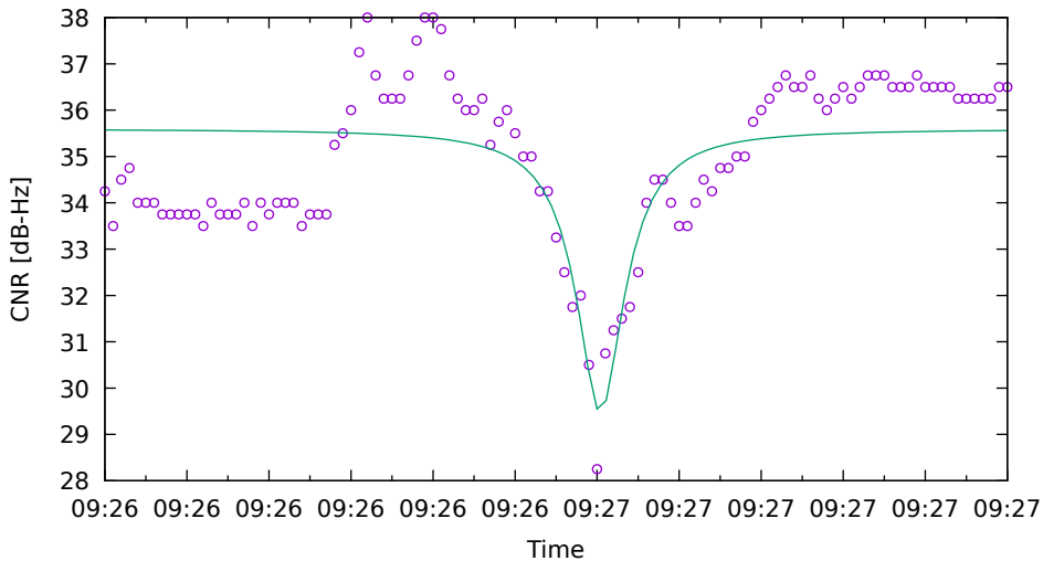
CNR fit for E34 on XiaomiMi8 - drive 6 (DOY262)
