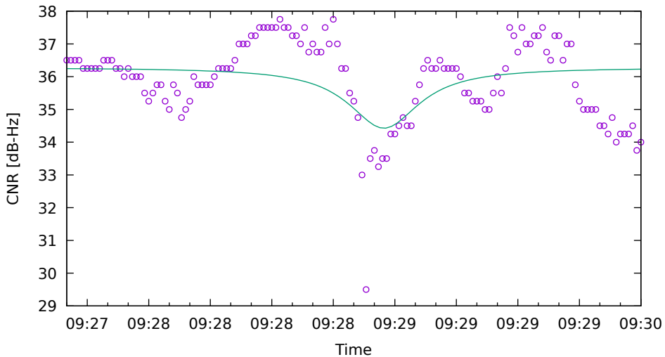
CNR fit for E34 on XiaomiMi8 - drive 7 (DOY262)
