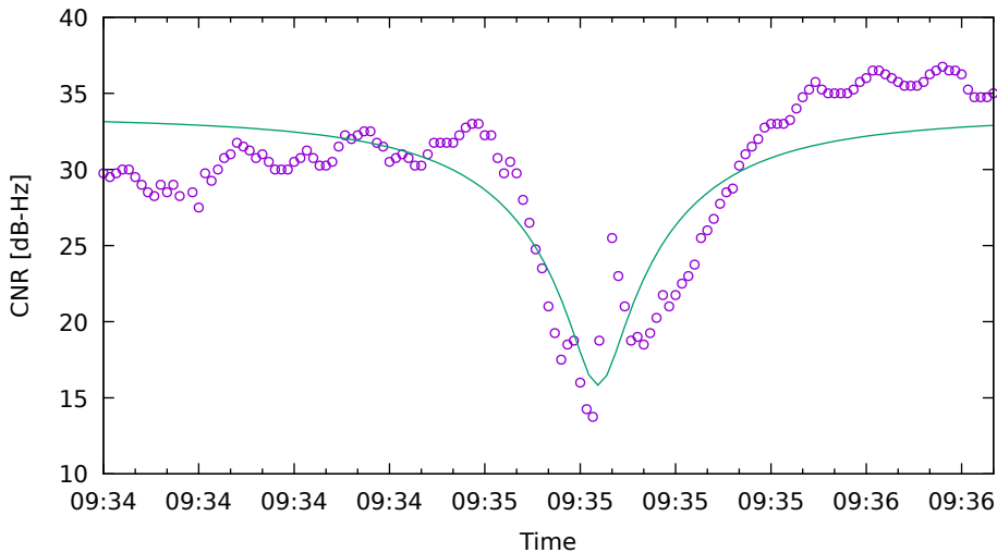
CNR fit for G01 on XiaomiMi8 - drive 10 (DOY262)
