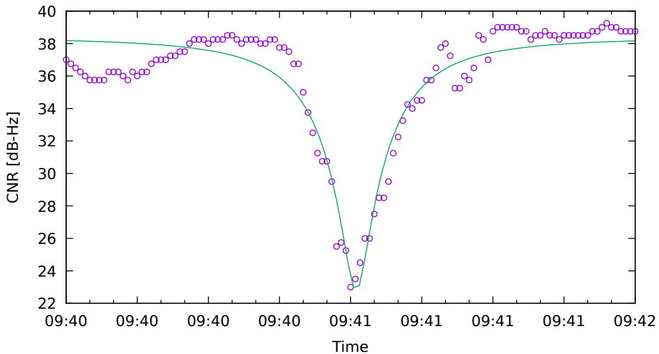
CNR fit for G01 on XiaomiMi8 - drive 13 (DOY262)
