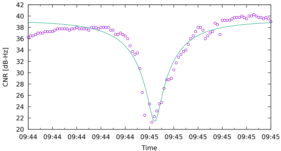
CNR fit for G01 on XiaomiMi8 - drive 15 (DOY262)
