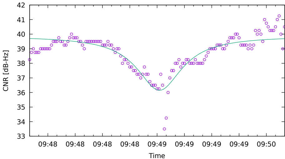
CNR fit for G01 on XiaomiMi8 - drive 17 (DOY262)
