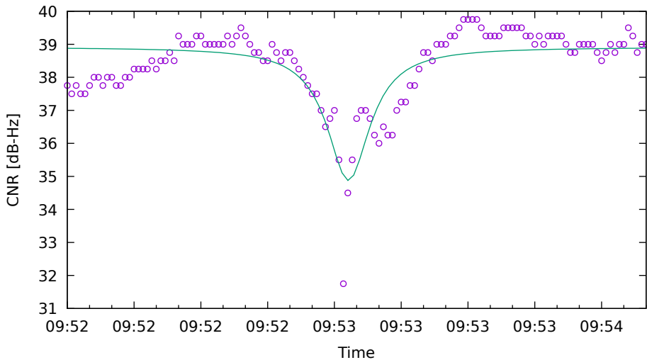
CNR fit for G01 on XiaomiMi8 - drive 19 (DOY262)
