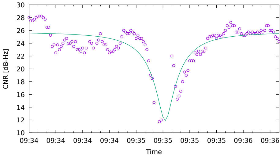
CNR fit for G03 on XiaomiMi8 - drive 10 (DOY262)
