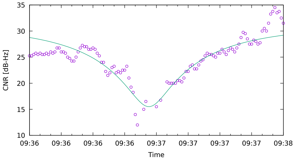
CNR fit for G03 on XiaomiMi8 - drive 11 (DOY262)
