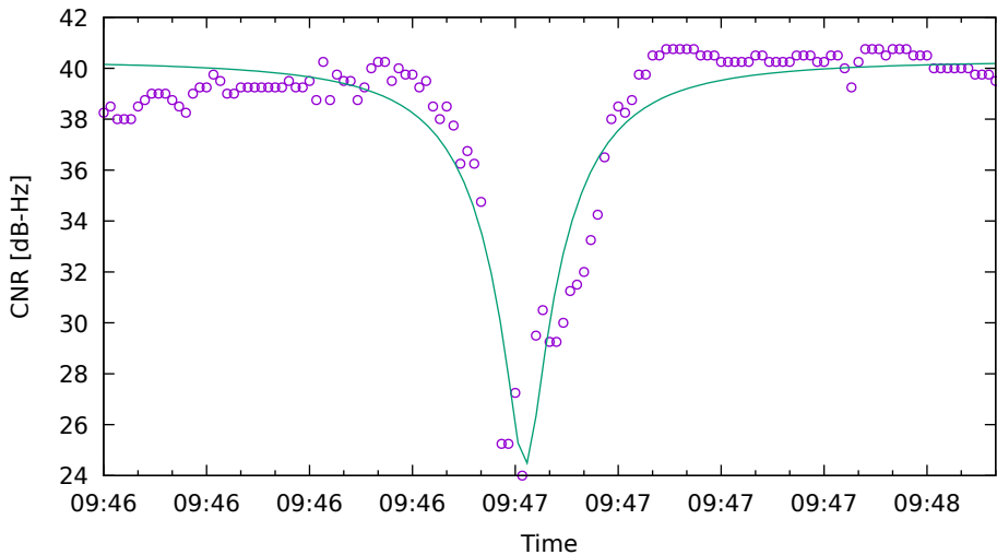
CNR fit for G03 on XiaomiMi8 - drive 16 (DOY262)
