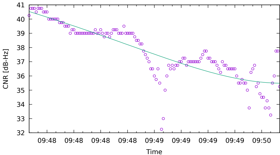
CNR fit for G03 on XiaomiMi8 - drive 17 (DOY262)
