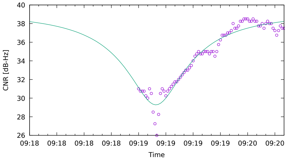
CNR fit for G03 on XiaomiMi8 - drive 2 (DOY262)
