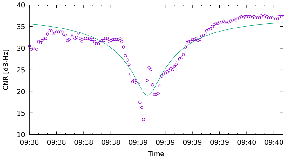
CNR fit for G08 on XiaomiMi8 - drive 12 (DOY262)
